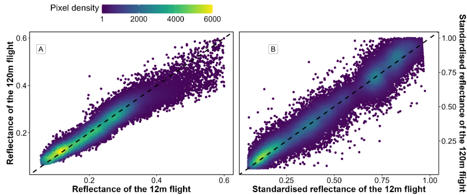
Figure 4: Comparison of reflectance retrieved from both low-altitude and high-altitude flights over a common area. The black dashed line represents a 1 to 1 relationship. Left (A) plots raw data and right (B) plots standardized data (Equation 1).
